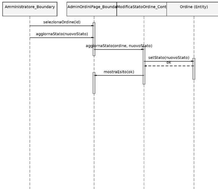
Sequence Diagram - UC9 ModificaStatoOrdine
