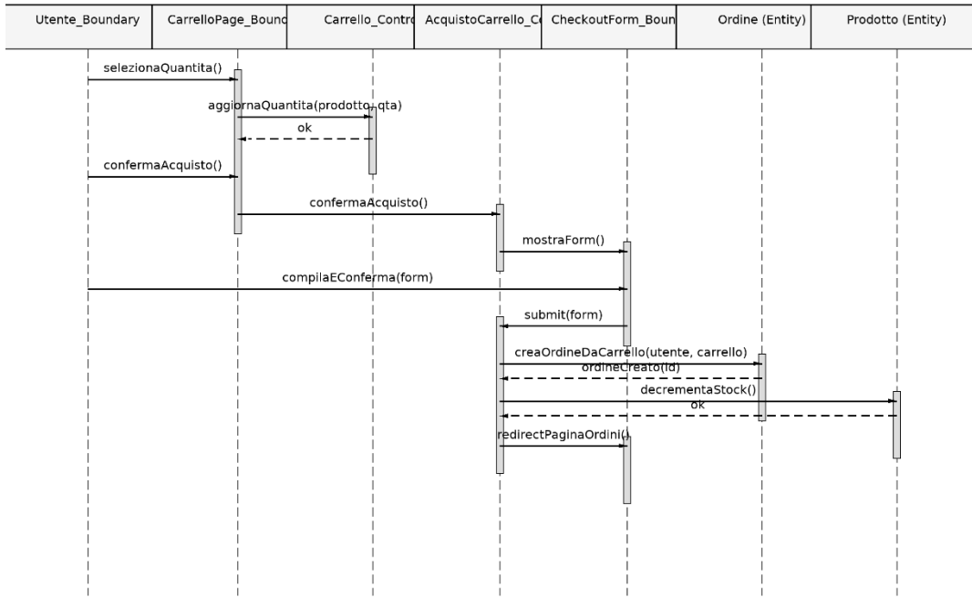
Sequence Diagram - UC4 AcquistoDaCarrello
